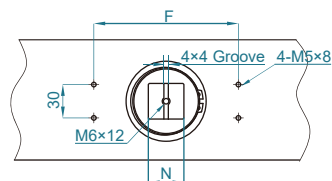
VDI/VDE 3845 Top connection
