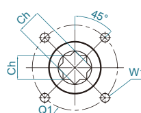
ISO5211 - DIN3337 Bottom view
